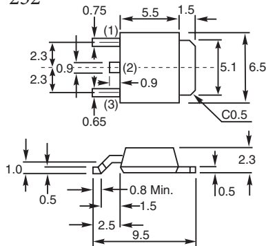
DPAK TO-252
