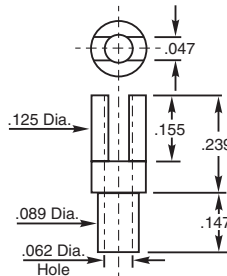
Bifurcated Terminal
