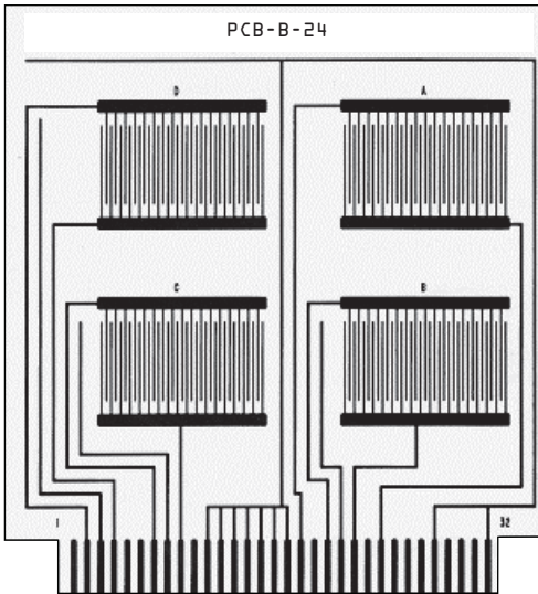
PCB-B-24 Standard Test Board
