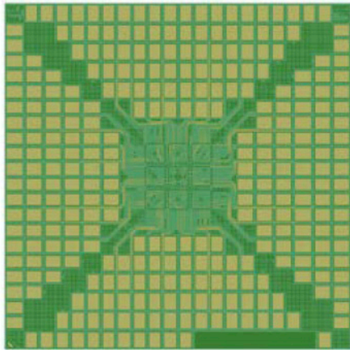
TOP SIDE VIEW (for 1 × 1chip, 3 × 3chip)
