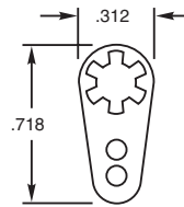
Pierced Terminal
