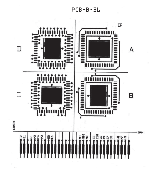
PCB-B-36 Standard Test Assembly
