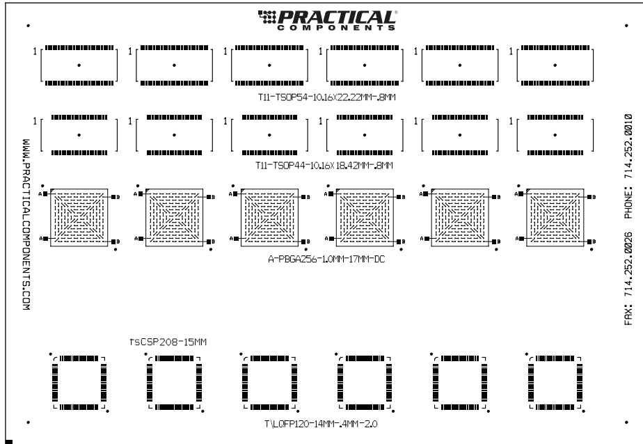
Bottom view Board size: 8" x 5.5", .062" thick.
