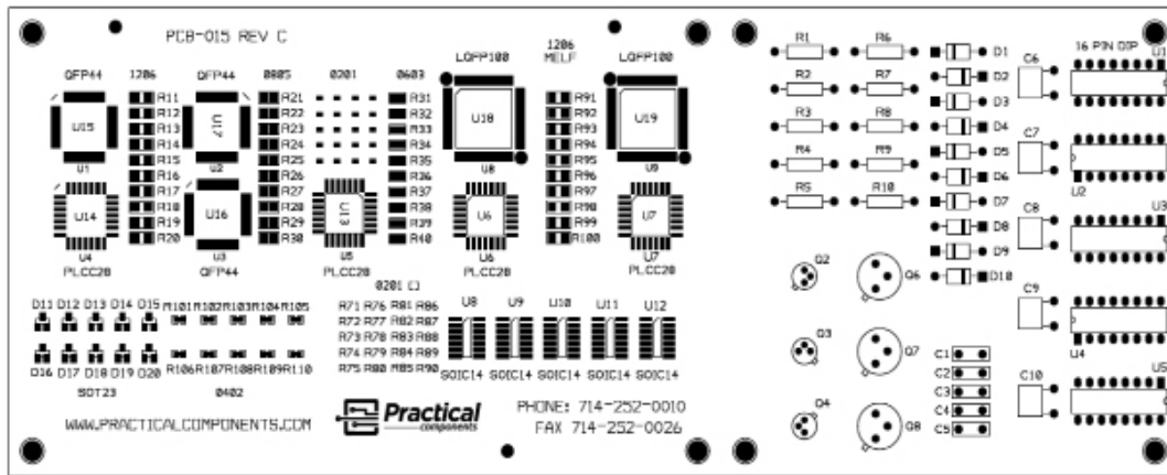
Board size: 9.850" x 3.750", .062" thick.
