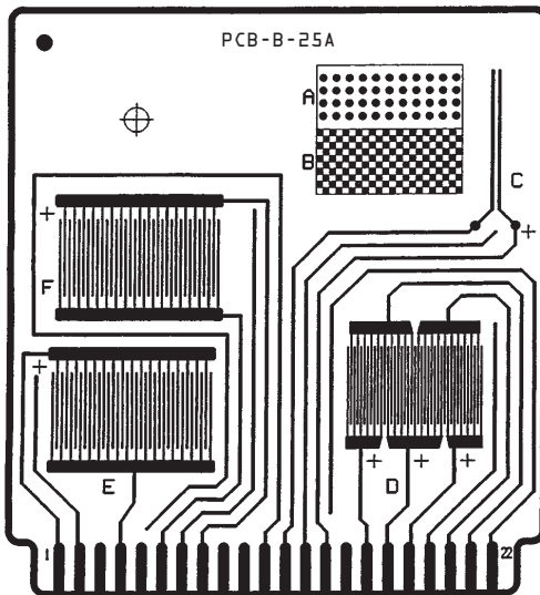
PCB-B-25A Standard Test Board
