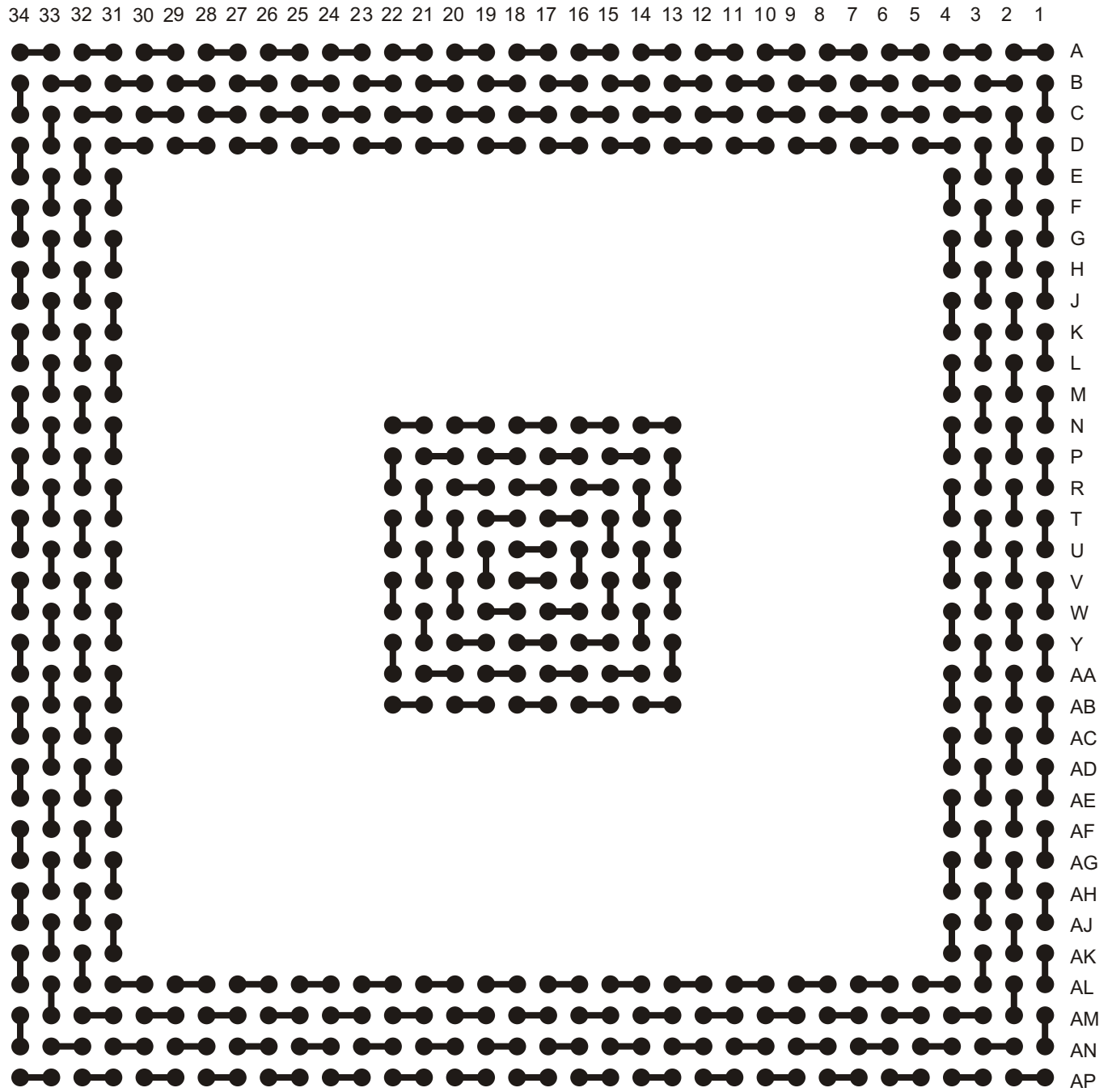
A-PBGA580-1.0mm-35mm-DC
