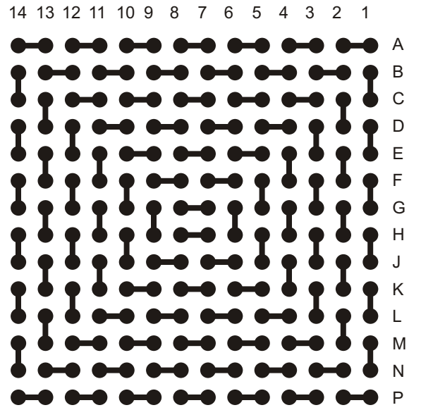
A-PBGA196-1.0mm-15mm Ball View
