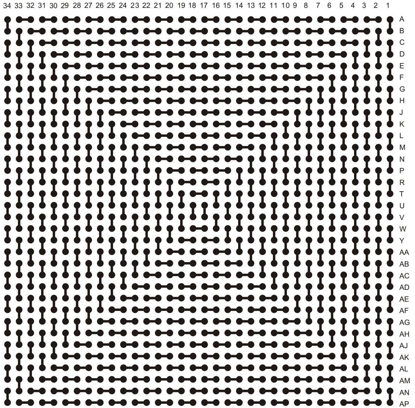
A-PBGA1156-1.0mm-35mm
