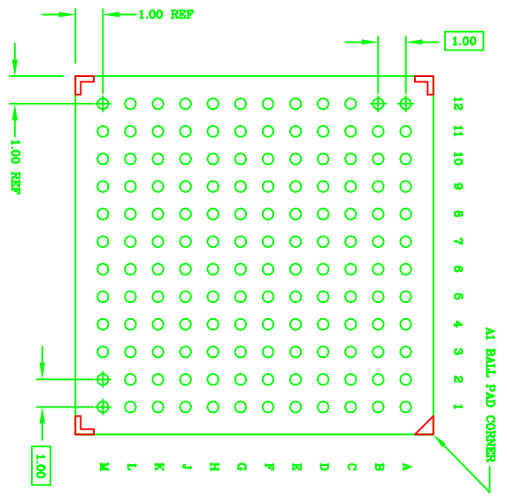
BOTTOM VIEW (144 SOLDER BALLS)
