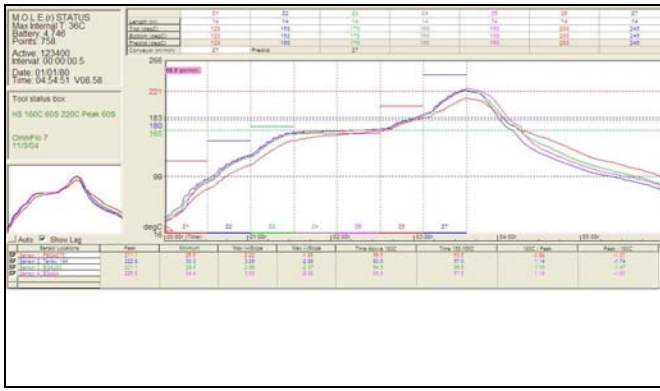
Figure 5. Soak profile for Tin-Lead alloy. Soak time is 60 seconds at 160 C. Peak temperature is 210-220 C.
