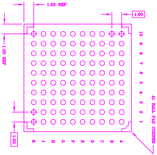
BOTTOM VIEW (100 SOLDER BALLS)
